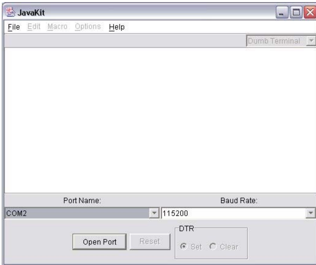
Figure 3. JavaKit Interface
